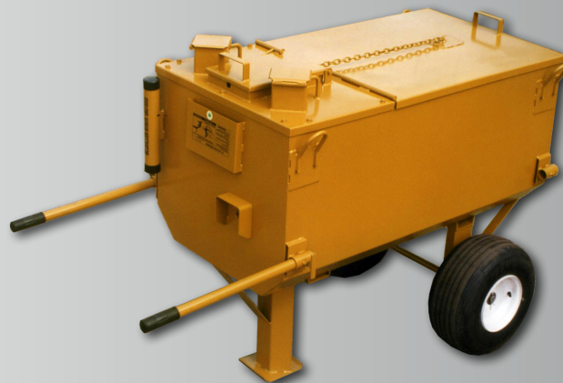
100 Gallon Patch Kettle (On-Deck)
