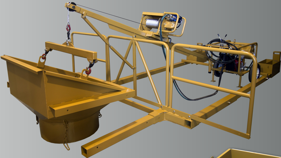
Trash Chute - Frame Assembly, Hoist, & Chute *Note - this is a rendered image.
