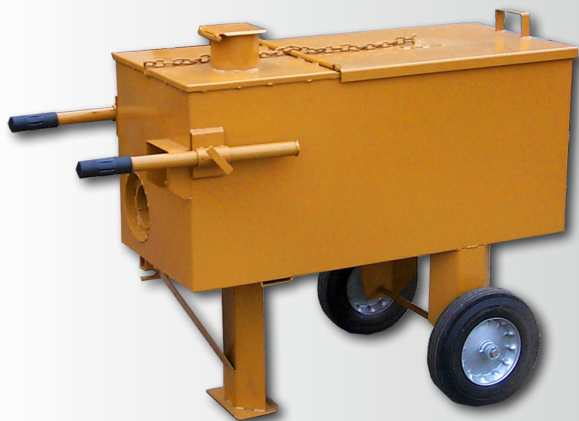
45 Gallon Patch Kettle (Standard)
