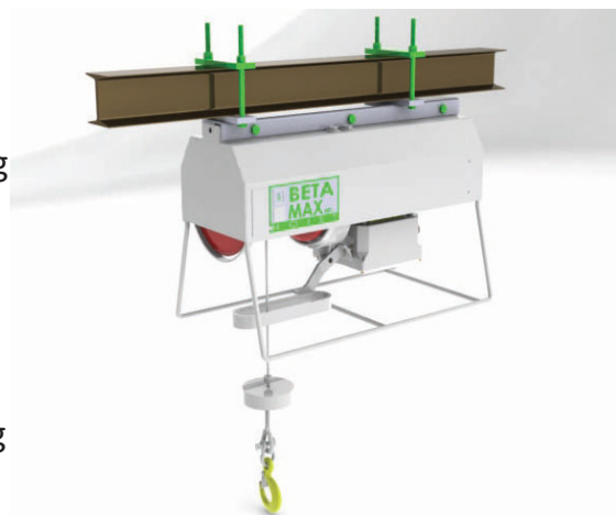
Fixed I-Beam: 60-8
